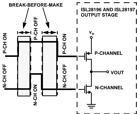
FIGURE 43. MAKE-BEFORE-BREAK ACTION OF THE OUTPUT STAGE
